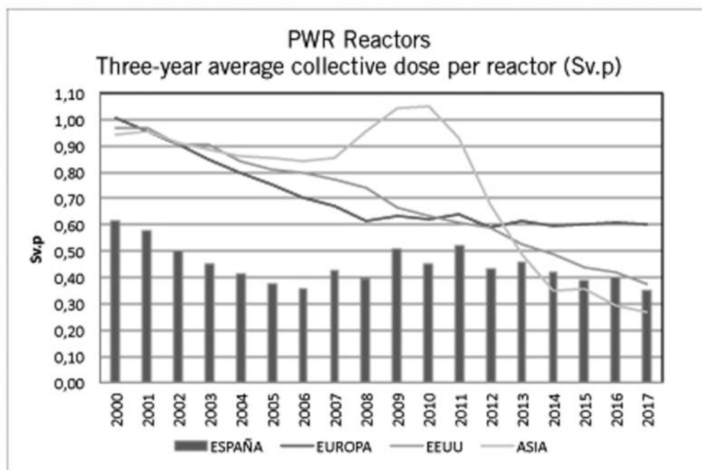
Figure 15.A.1 Average three-yearly collective dose (Sv-person) for PWR type reactors. International Comparison
