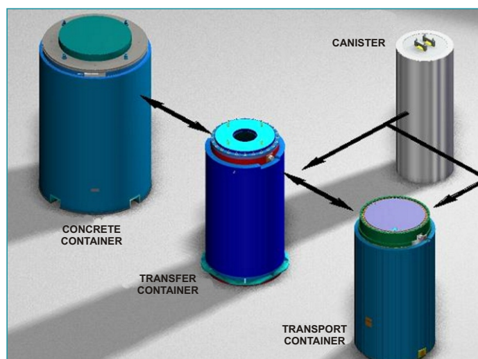
Figure 5. Storage system.
