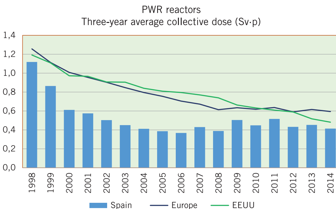
Figure 15.A.1 Three-year average collective dose (Sv·person) for PWR reactors. International comparison
