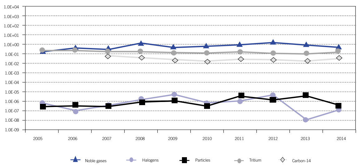
Figure 3.2.2.2. Gaseous radioactive effluents from PWR plants. Normalised activity (GBq/GWh)
