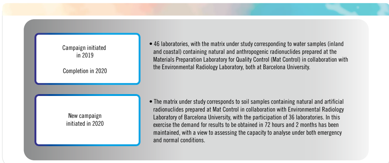
Figure 5.2.2.1. Intercomparison campaigns
