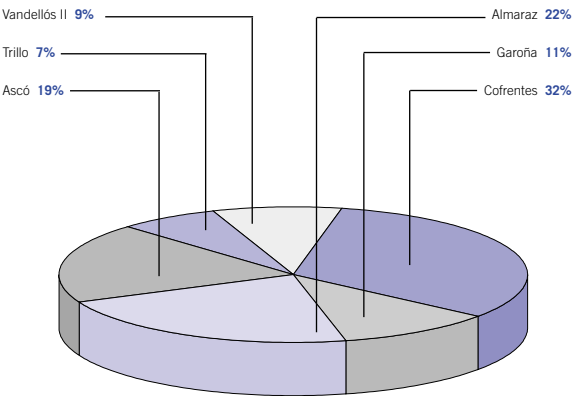
Figure 6.2.1. Distribution of the 2,859 conditioned radioactive waste packages at the operating nuclear power plants in 2016
