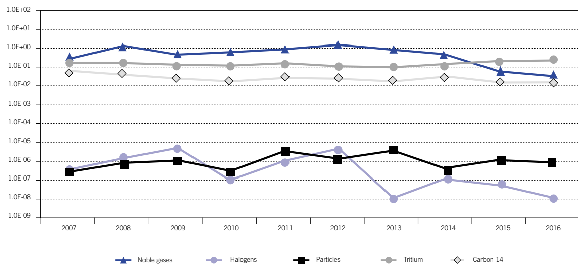
Figure 3.2.2.2. Gaseous radioactive effluents from PWR plants. Standardised activity (GBq/GWh)
