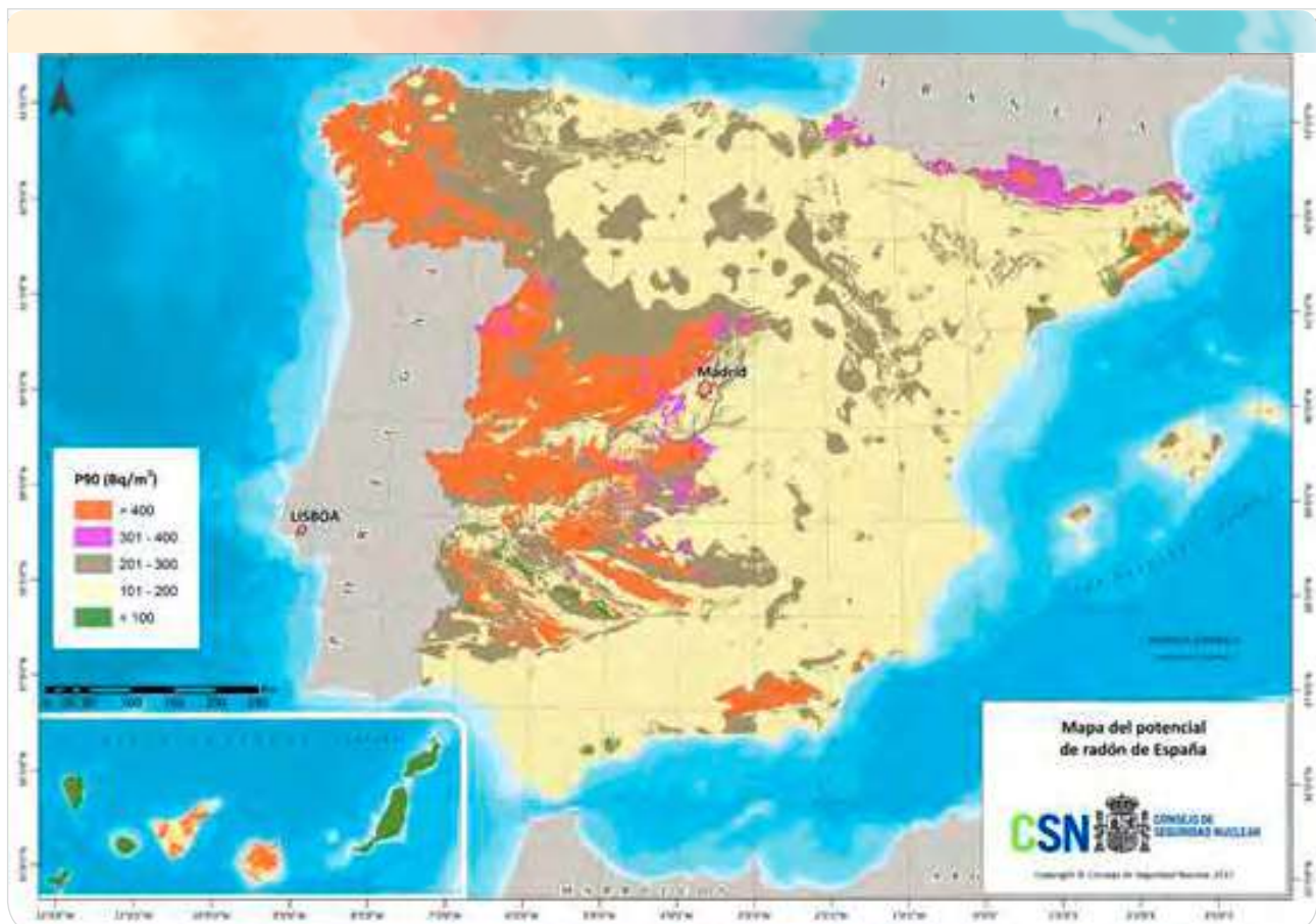
Figure 5.3.1. Map of Spain's radon potential
