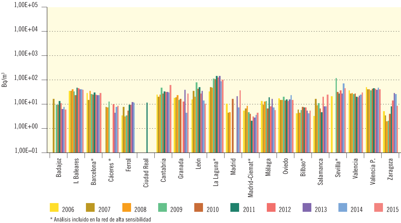
Figura 3.10a. Agua potable
