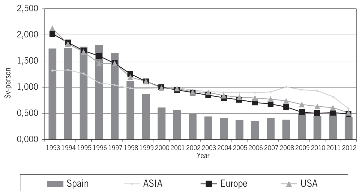
Figura 15.A.1 Average triennial collective dose (Sv/person) for PWRs. International comparison.
